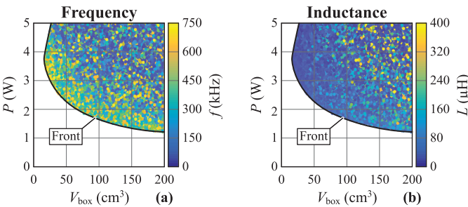
FIGURE 17. Obtained Pareto plots and fronts (boxed volume vs. losses) with the ANN-based workflow. (a) Operating frequency. (b) Inductance value.
