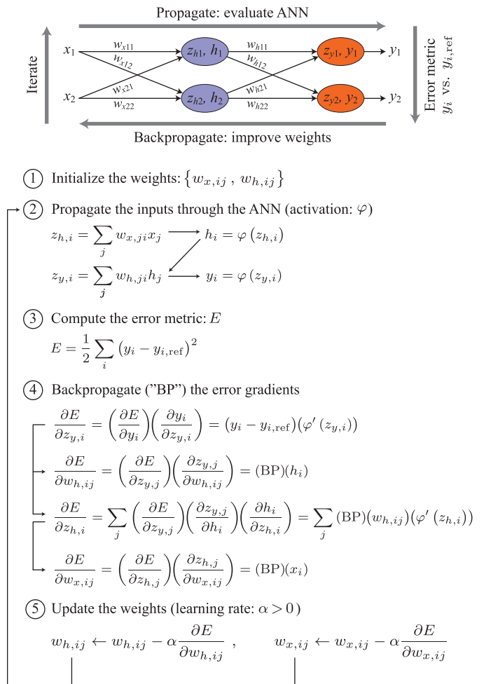
FIGURE 6. Basic ANN training algorithm based on the propagation of the inputs and the backpropagation of the errors (supervised learning).
