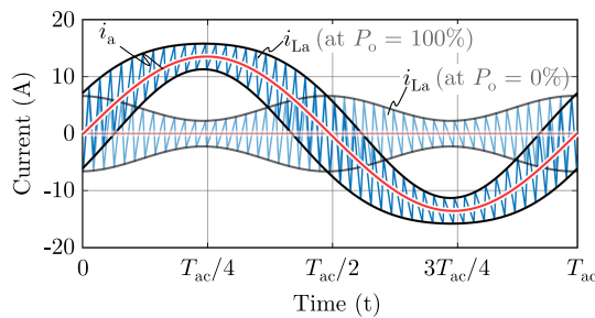
FIGURE 9. Simulated inductor ( i_{L,a} ) and average output ( i_a ) current waveforms in a CCM bridge-leg with a switching frequency of 48 kHz and an inductor of 315 \mu\text{H} at full load and zero load.
