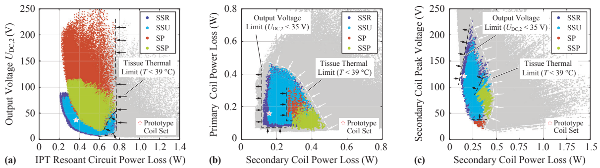
Figure 6: Comparison of the considered IPT resonant circuit topologies for maximum power transfer and maximum coil coupling, including the indicated prototype IPT coil set with the specifications given in Fig. 7(d), operated as SSU system. (a) Calculated total power loss. (b) Calculated primary and secondary side coil power loss, when the system output voltage is limited to 35 V. (c) calculated secondary side coil peak voltage with respect to the secondary side coil power loss with the same output voltage limitation.
