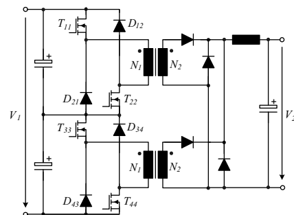
Fig.1. Schematic of a telecom power supply, which is used for investigating different cooling methods.
