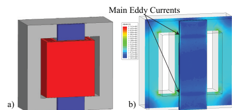
Fig. 11. (a) 3D model used in the FEM-simulation. (b) Result of the FEM simulation with magnetic flux density in the core and current density in the HTC.
