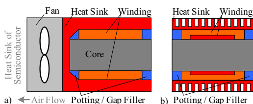
Fig. 4. (a) Transformer with special heat sink. (b) Side view of the heat sink including transformer.
