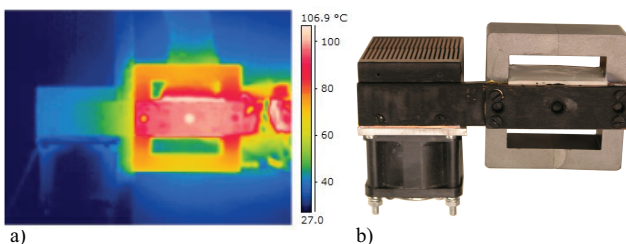
Fig. 8. (a) Measurement of temperature distribution with thermo camera for the setup with optimised copper heat sink (10) shown in (b).
