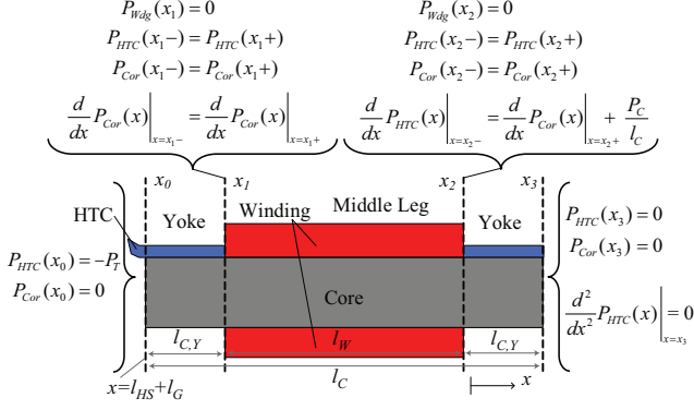
Fig. 6. Initial conditions/constraints for the differential equations of the temperature distribution in the HTC.
