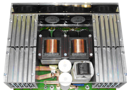
Fig.2. Photo of a 10kW telecom power supply with conventional forced air cooled magnetic devices (schematic in fig. 1).
