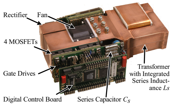
Fig. 12. Application of the indirect air cooling to a 5kW telecom power supply with 10\text{kW}/\text{dm}^3 and 1U height ( H \times W \times L = 40 \times 80 \times 155\text{mm} ).
