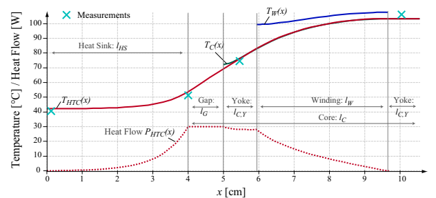
Fig. 9. Distribution of temperature and heat flow in a HTC made of copper for T_{Ambient} = 40^\circ C .
