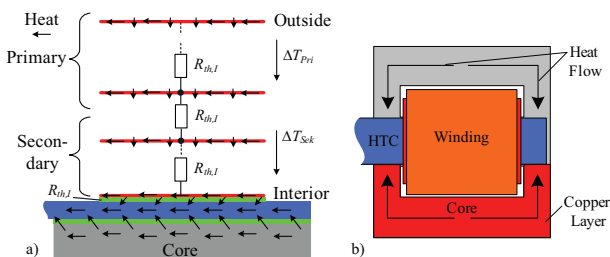
Fig. 7. (a) Heat flow in the winding from the single layers to the HTC via the insulation ( R_{th,I} ) and (b) Heat flow in the core improved by copper layer.
