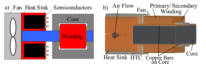
Fig. 3. Example for thermally connecting a heat sink and a transformer with single sided cooling in (a) and parallel connection of two HTCs for double sided cooling in (b) (top+bottom).
