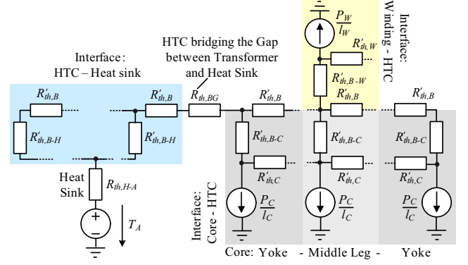
Fig. 5. Distributed thermal model of the cooling system shown in figure 3 with the heat sink on the left hand side, a gap between heat sink and transformer and the transformer with winding on the right hand side.
