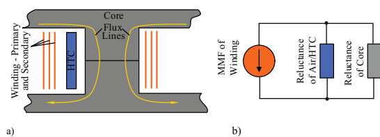
Fig. 10. (a) Middle leg of a transformer with a HTC in the window. (b) Simplified magnetic equivalent circuit of the transformer.
