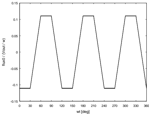
Fig. 11. Waveform of the stray flux
