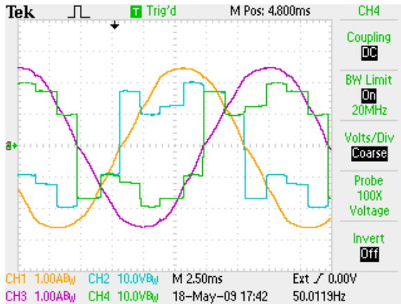
Fig. 13. Waveforms of i_{A1} , v_{A1} , i_{A2} , and v_{A2} , 3 \times 1\Phi
