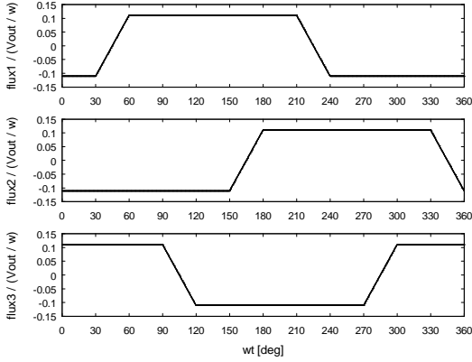
Fig. 9. Waveforms of the limb fluxes
