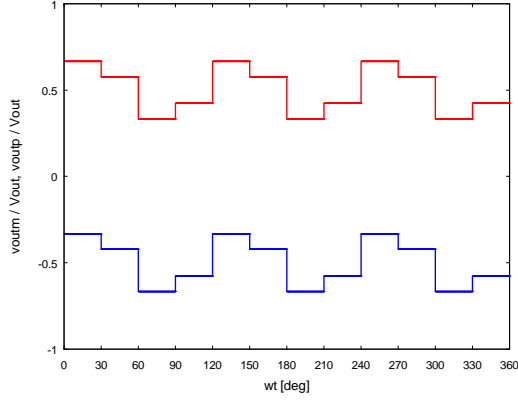
Fig. 3. Waveforms of v_{OUTP} (red) and v_{OUTM} (blue)
