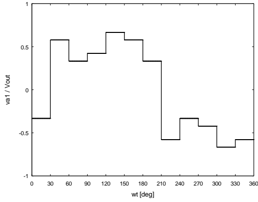
Fig. 4. Waveform of v_{A1}
