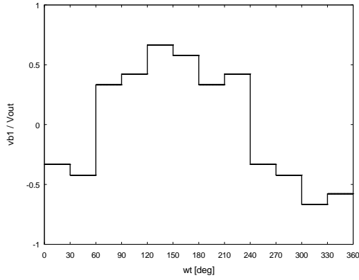
Fig. 5. Waveform of v_{B1}
