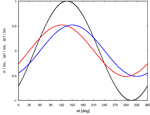
Fig. 2. Waveforms of i_1 (black), i_{A1} (red), and i_{B1} (blue) which is used to determine v_{OUTP} and v_{OUTM} .
