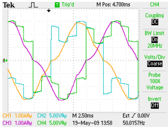
Fig. 12. Waveforms of i_{A1} , v_{A1} , i_{A2} , and v_{A2} , 3\Phi
