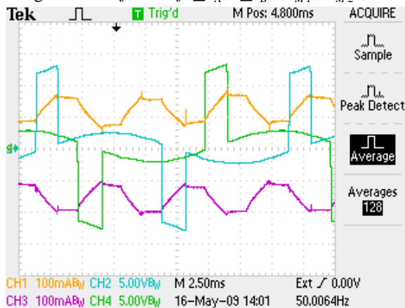
Fig. 15. Waveforms of \sum i_A , \sum i_B , v_{M1} , v_{M2} , 3 \times 1\Phi
