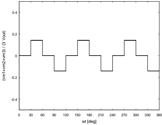
Fig. 10. Zero sequence of the voltages across the magnetizing windings
