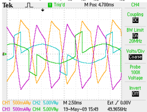
Fig. 14. Waveforms of \sum i_A , \sum i_B , v_{M1} , v_{M2} , 3\Phi
