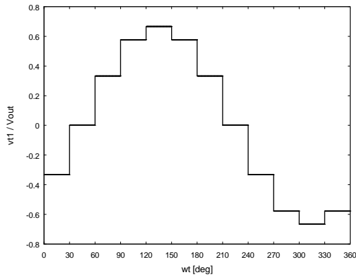
Fig. 6. Waveform of v_{T1}
