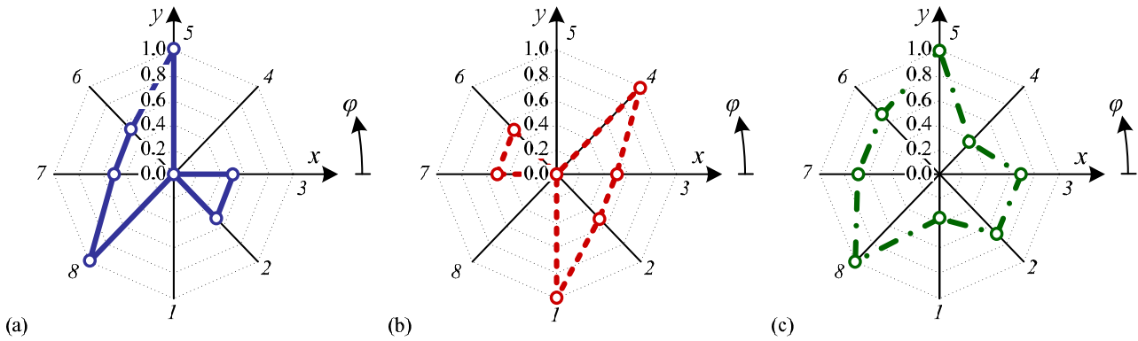
Fig. 8 Copper loss ratio P_{cuc} / P_{cus} for each claw: (a) \theta_d / \theta_b = 1, \varphi = 0^\circ ; (b) \theta_d / \theta_b = 1, \varphi = 22.5^\circ ; (c) \theta_d / \theta_b = 4, \varphi = 0^\circ ;
