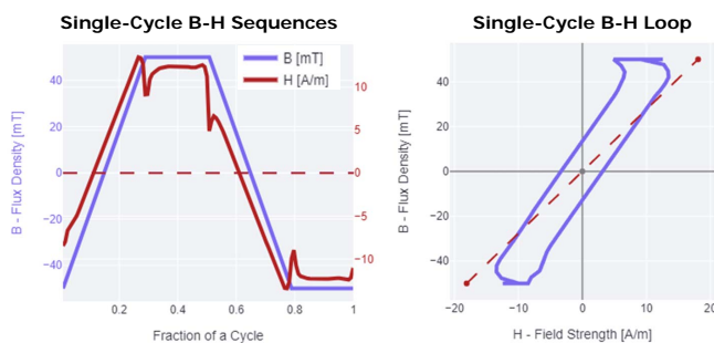
FIGURE 3. An example data sample offered in the MagNet Challenge. This data point describes the B-H loop of N87 material operating at 25°C, 200 kHz, and zero dc bias under a trapezoidal excitation. The volumetric core loss is 113.64 kW/m 3 under zero dc bias. Over 2,000,000 data points like this are available in the MagNet database for 15 different materials.
