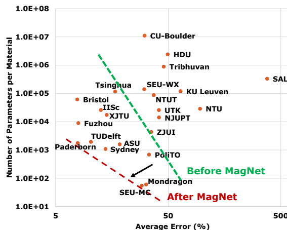
FIGURE 5. Average 95 th percentile error across the 5 materials, and average model number of parameters (size) of the 24 final submissions, together with the state-of-the-art (SOTA) Pareto fronts before and after the MagNet Challenge, estimated using the results reported in [30] as a benchmark. The minimum average 95 th percentile error reaches 7%, and the smallest model parameter size reaches 60. Both the model sizes and average errors are greatly reduced as a result of the community effort in the MagNet Challenge.
