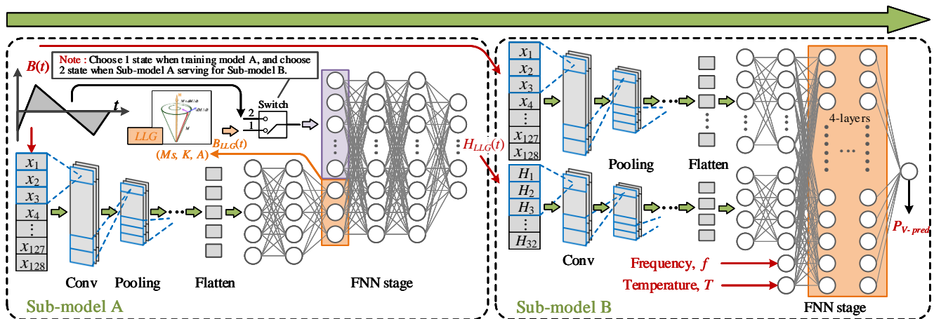
FIGURE 9. The two-stage PI-MFF-CN architecture developed by Southeast University SEU-WX.
